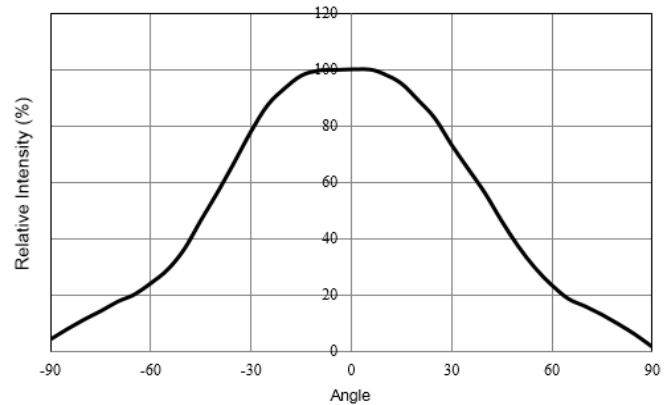
C3535X-FNAX (beam angle 90^{\circ} )
