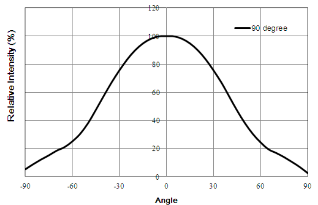
C3535X-JNAx series (beam angle 90°)
